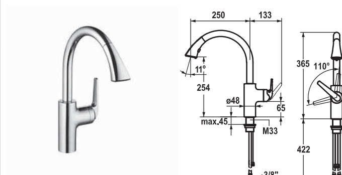
KWC-No. 10.061.004.000FL Finish all chrome A 250, flexible connection hoses
