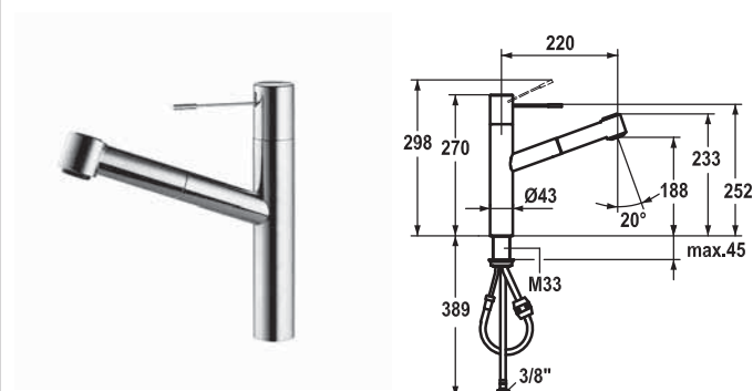
KWC-No. 10.151.033.000FL all chrome A 220, flexible connection hoses
