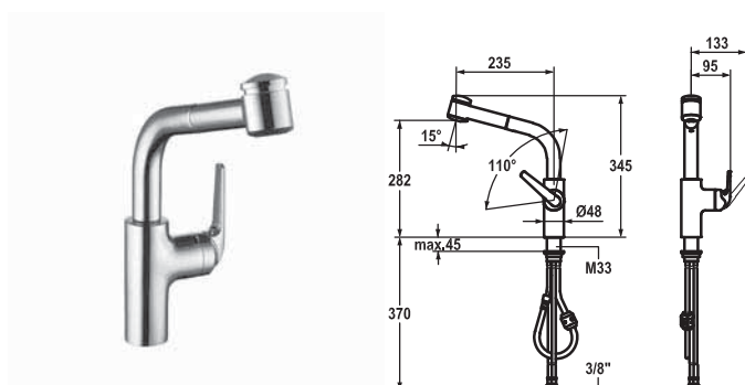
KWC-No. 10.061.003.000FL Finish all chrome A 235, flexible connection hoses
