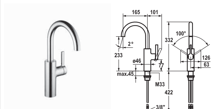
KWC-No. 10.181.992.000FL Finish all chrome A 165, flexible connection hoses
