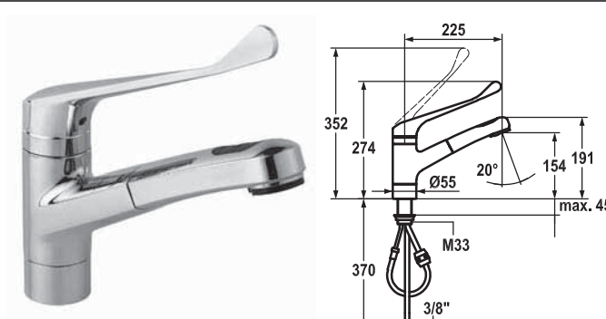
KWC-No. 10.071.033.000LLFL Finish all chrome A 225, flexible connection hoses, with long lever
