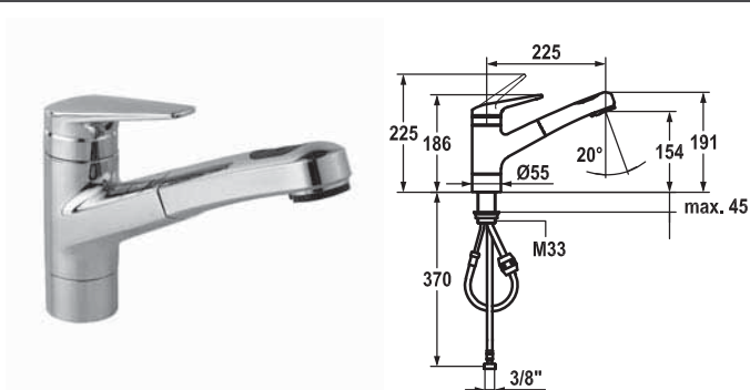
KWC-No. 10.071.033.000FL Finish all chrome A 225, flexible connection hoses
