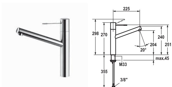
KWC-No. 10.151.023.000FL all chrome A 225, flexible connection hoses
