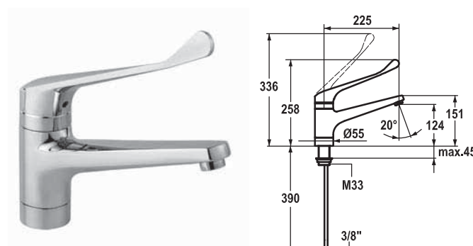
KWC-No. 10.071.023.000LLFL Finish all chrome A 225, flexible connection hoses, with long lever
