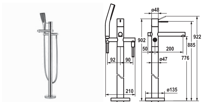
KWC-No. 20.151.094.000 all chrome A 200, with hand shower and hose
