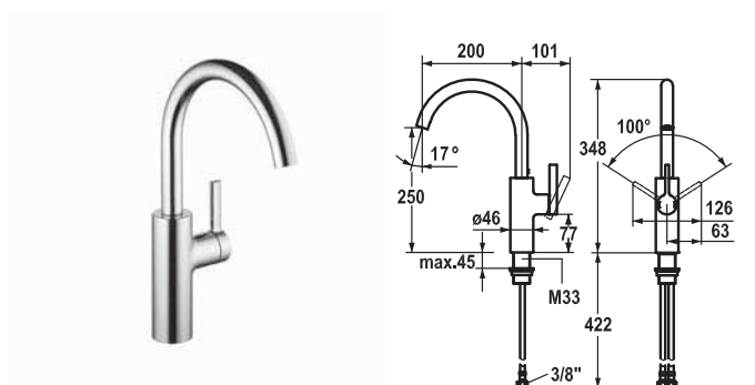
KWC-No. 10.181.012.000FL Finish all chrome A 200, flexible connection hoses
