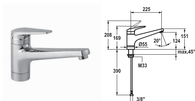
KWC-No. 10.071.023.000FL Finish all chrome A 225, flexible connection hoses
